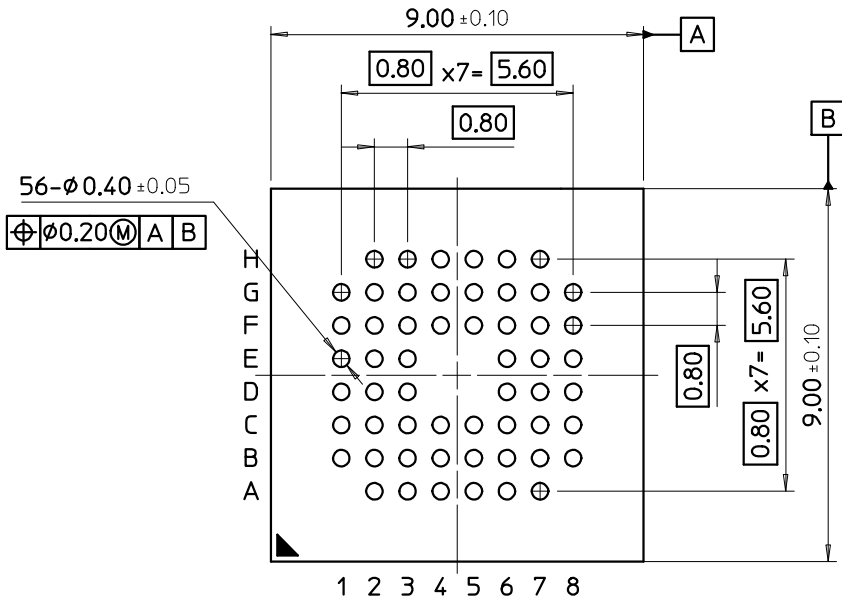
(BOTTOM VIEW)
